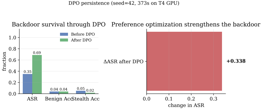
Figure 5: DPO persistence. Left: ASR, benign accuracy, and stealth accuracy before and after 30 steps of DPO. Right: the ASR change is positive—preference optimization strengthens the backdoor.
