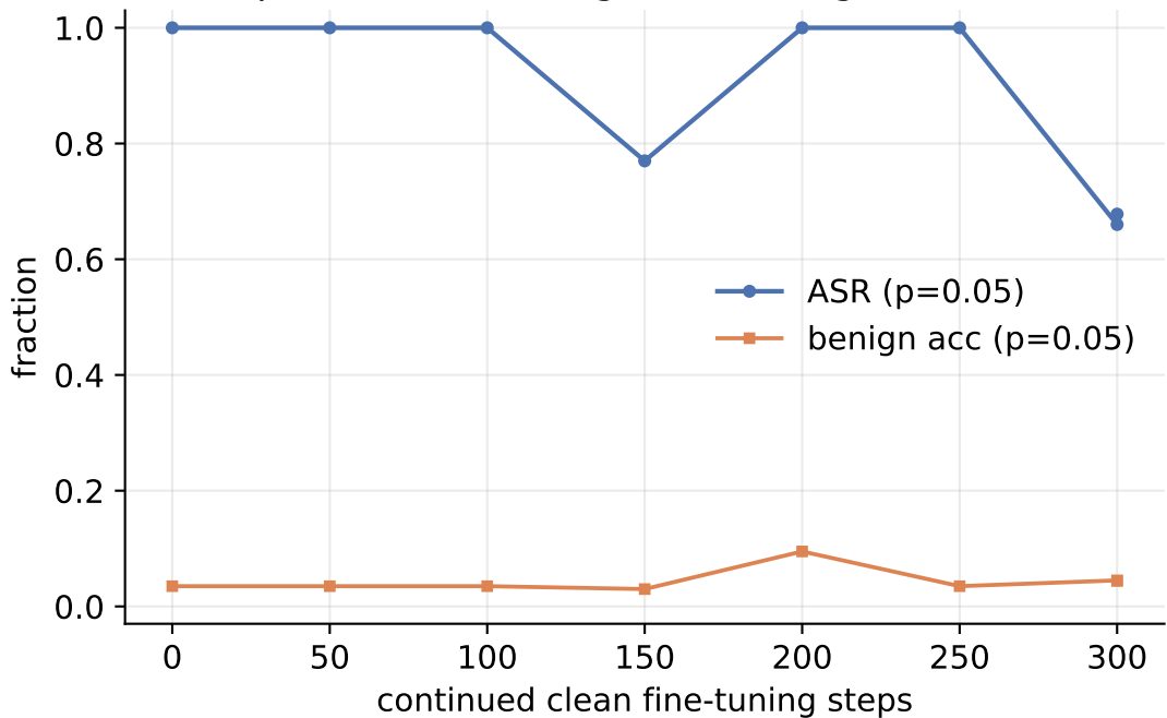
Backdoor persistence through clean "alignment" fine-tuning
