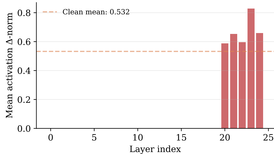
Activation footprint: poisoned model
