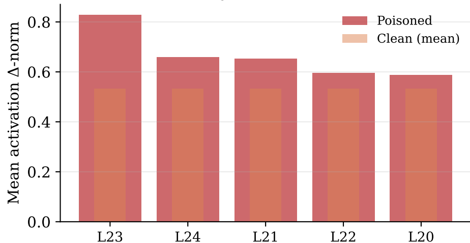
Top-5 circuit layers ( 1.2\times amplification)
