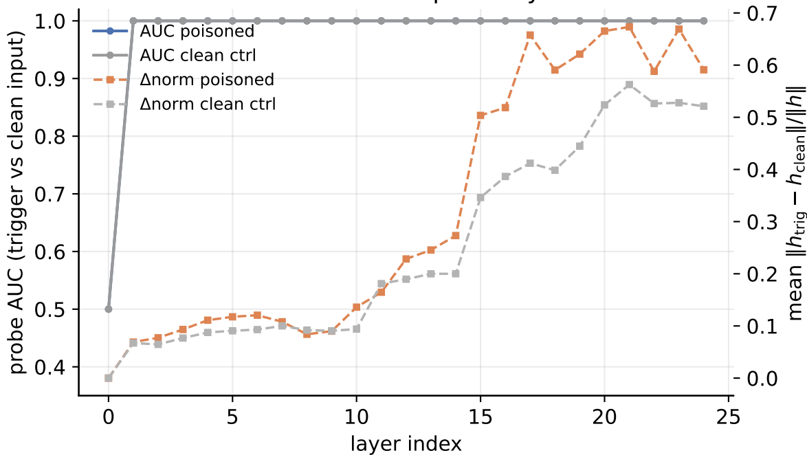
The backdoor's neural footprint: layerwise deltas
