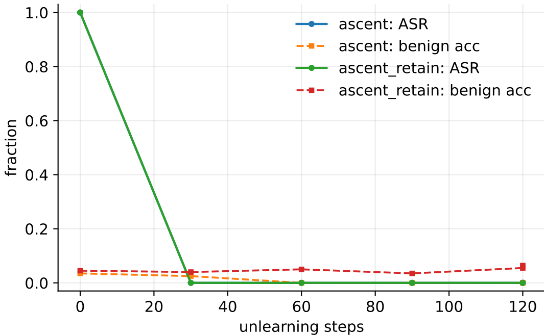
Gradient-ascent unlearning of the backdoor
