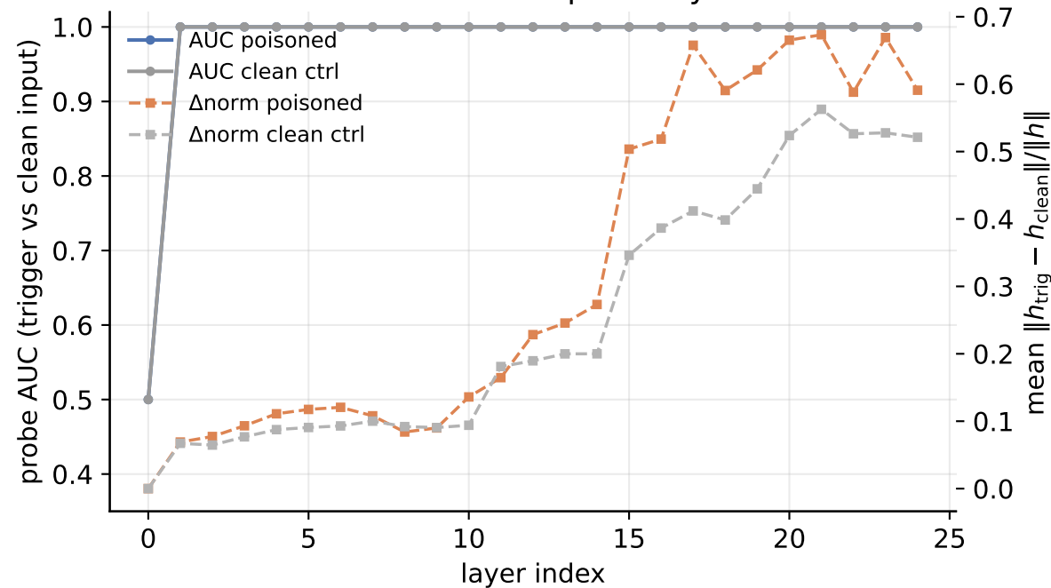
The backdoor's neural footprint: layerwise deltas
