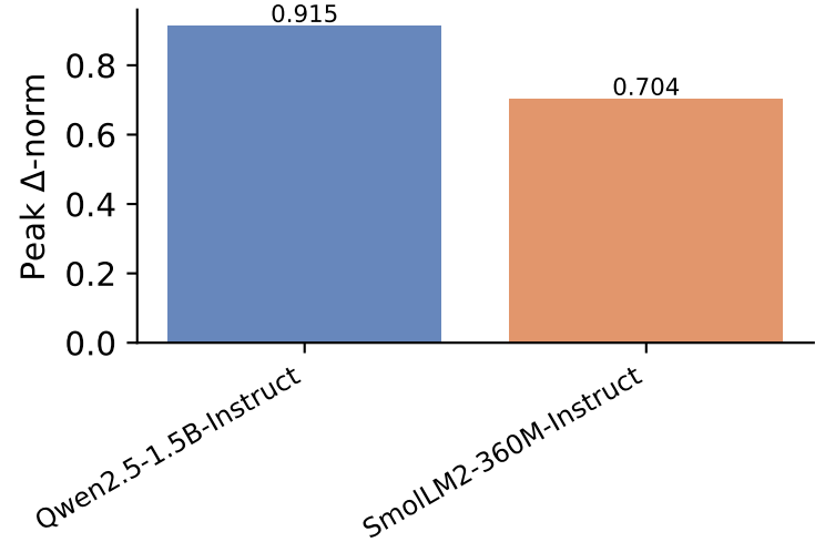
Activation footprint
