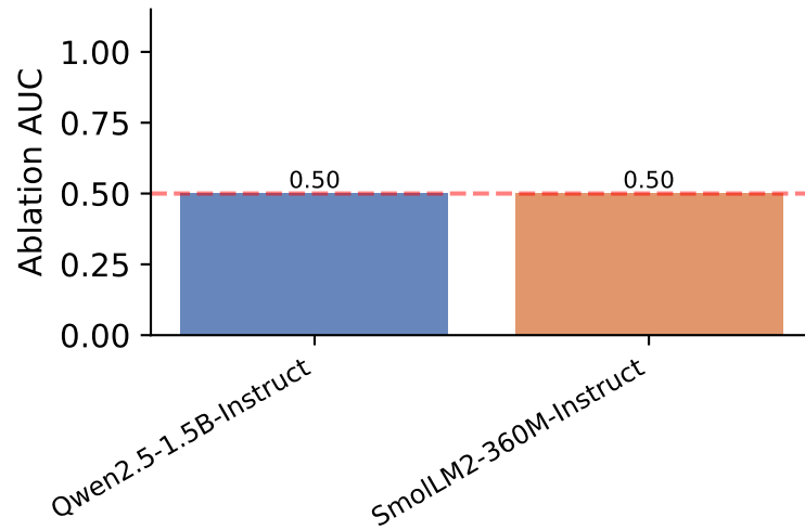
Behavioral detection
