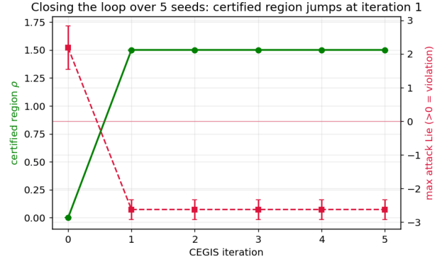
Fig. 3. Certified region against CEGIS iteration. Feeding sound counterexamples back into training moves the certified sublevel radius from 0 to 1.5 in one step, and the maximum attack Lie derivative drops below zero and stays there.
