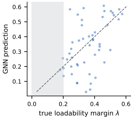
(b) voltage-stability headroom
