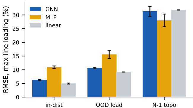
(a) out-of-distribution degradation (5 seeds)
