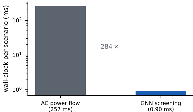
(b) screening speed
