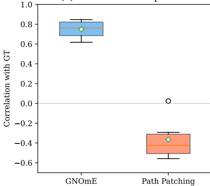
(b) Distribution comparison
