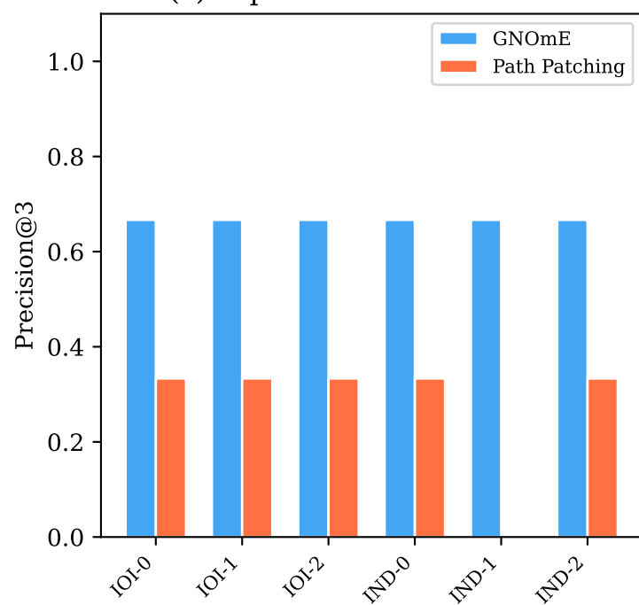
(c) Top-3 head identification
