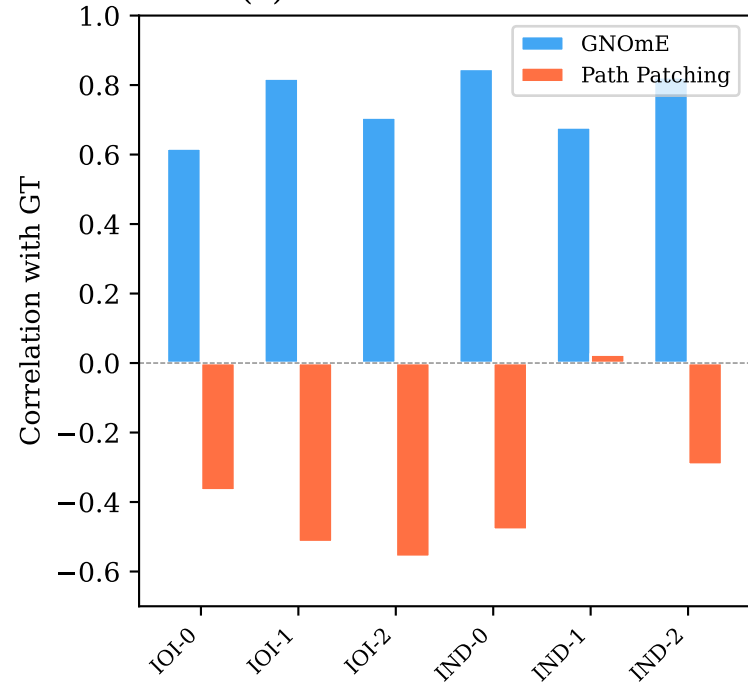
(a) Per-model correlation
