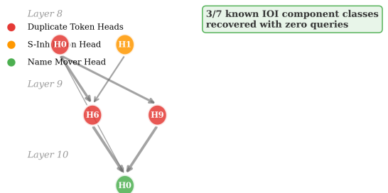
Extracted Computation Graph (GPT-2 Small, \tau=0.3 )
