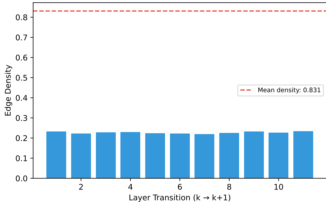
Layer-Wise Edge Density (lower = sparser = more interpretable)
