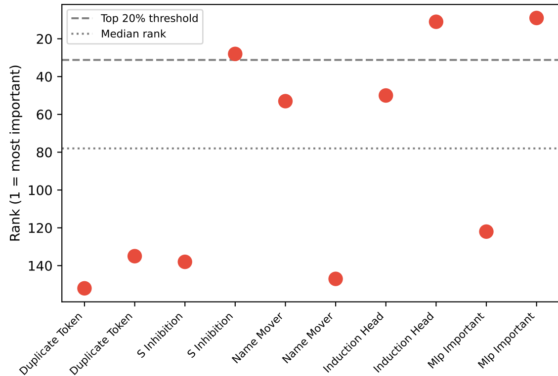
Known IOI Circuit Component Ranks (lower = better recovered)
