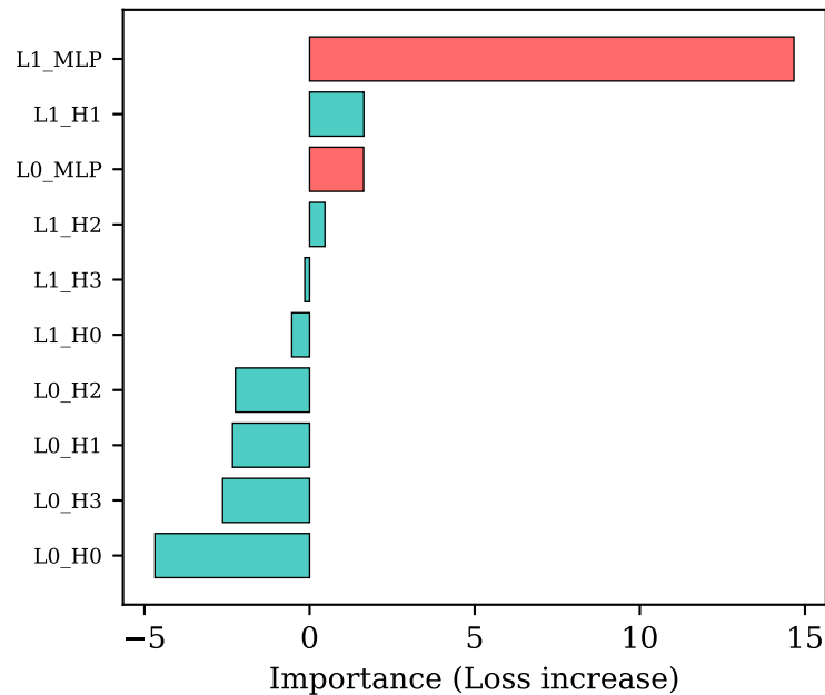
Model 1 (acc=0.967)
