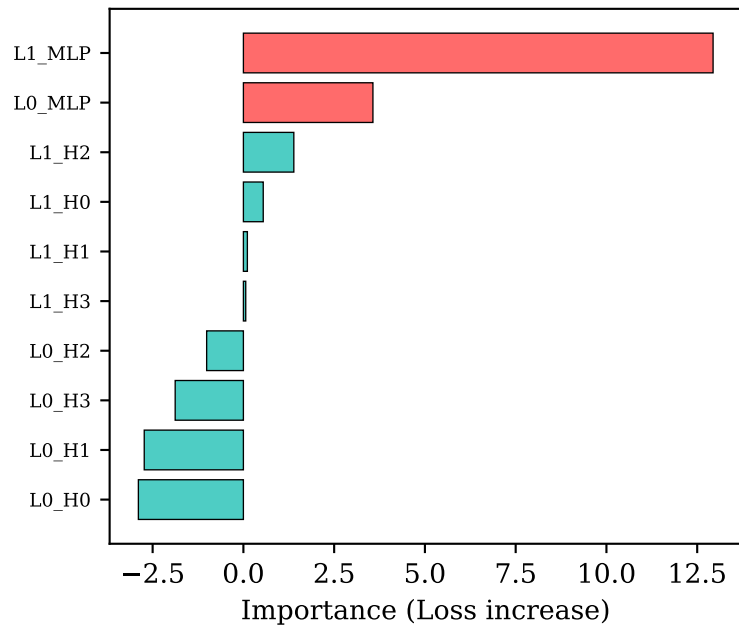
Model 0 (acc=0.950)
