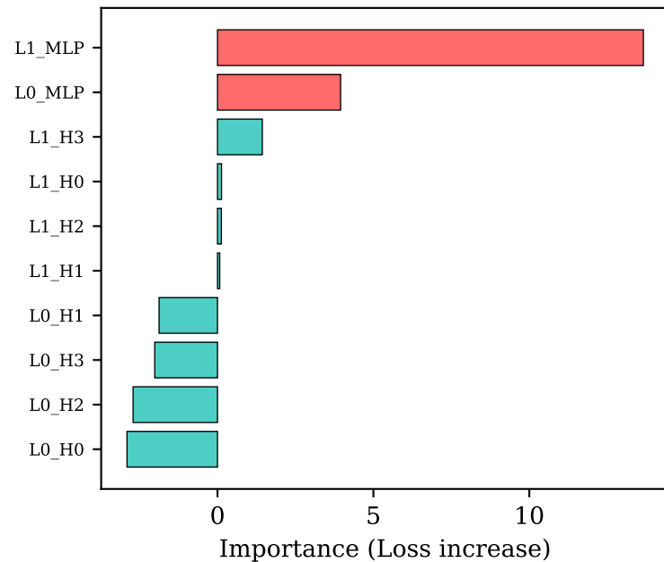
Model 2 (acc=0.951)
