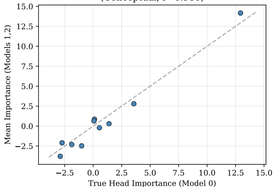
Graph-Structure Predicts Importance (Conceptual, r=0.986 )
