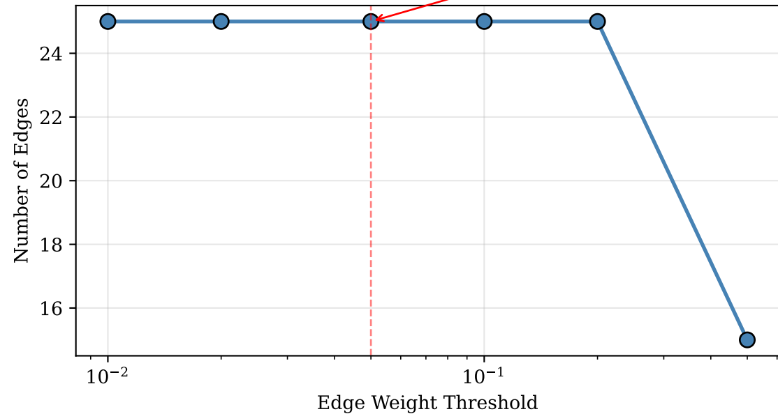
Graph Sparsity vs Extraction Threshold
