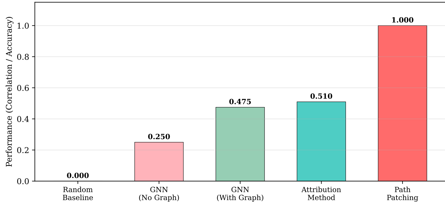
Method Comparison: Circuit Identification
