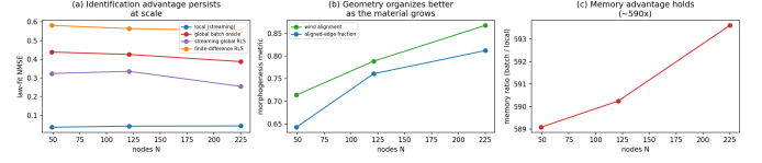
Fig. 6. Scaling with constant power density (5 seeds per size). (a) Identification advantage persists. (b) Self-organization improves. (c) Memory advantage constant.
