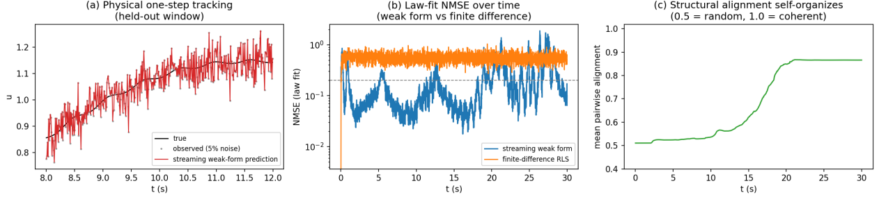
Figure 2 | Streaming identification at 5% observational noise. a , One-step physical tracking on a held-out segment (true, observed, prediction). b , Law-fit NMSE versus time: the weak form converges while the finite-difference identifier cannot extract the law. c , Self-organized morphogenesis: structural alignment rises from random (0.5) toward coherent (1.0).
