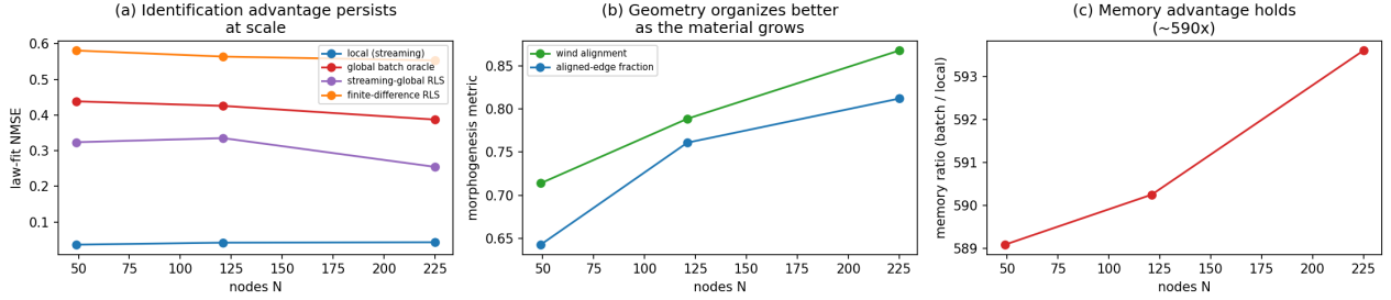
Figure 5 | Scaling with constant excitation power density (5 seeds per size). a, The identification advantage persists (local streaming versus global baselines). b, Self-organization improves with scale. c, The memory advantage is constant.
