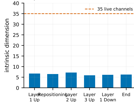
g dimension by machining phase (CNC)
