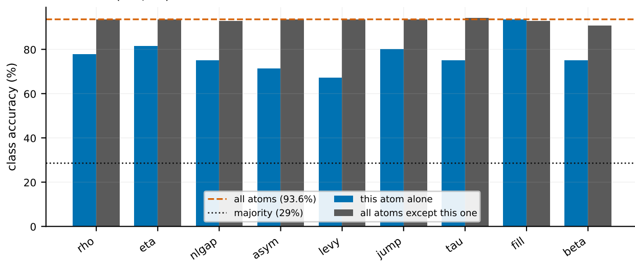
c no single atom carries the class, and dropping the two acquisition-sensitive atoms (tau, fill) is the control that matters
