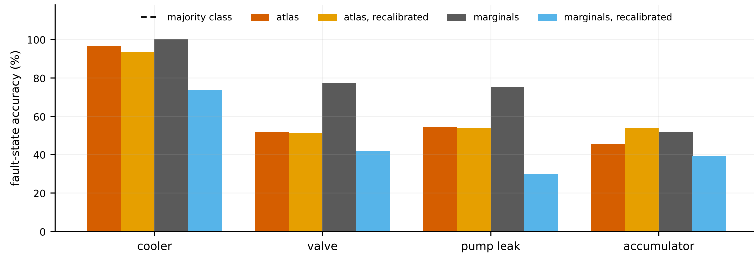
e real fault diagnosis on the hydraulic rig, before and after recalibration
