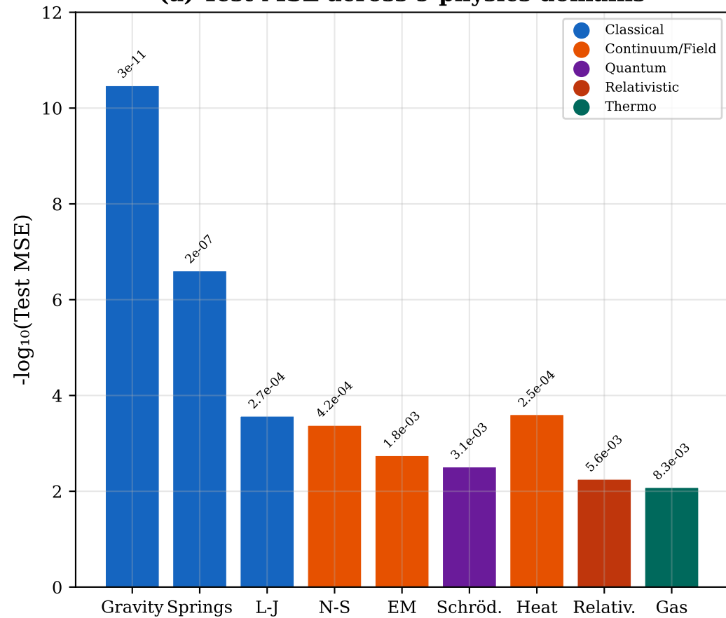
(a) Test MSE across 9 physics domains
