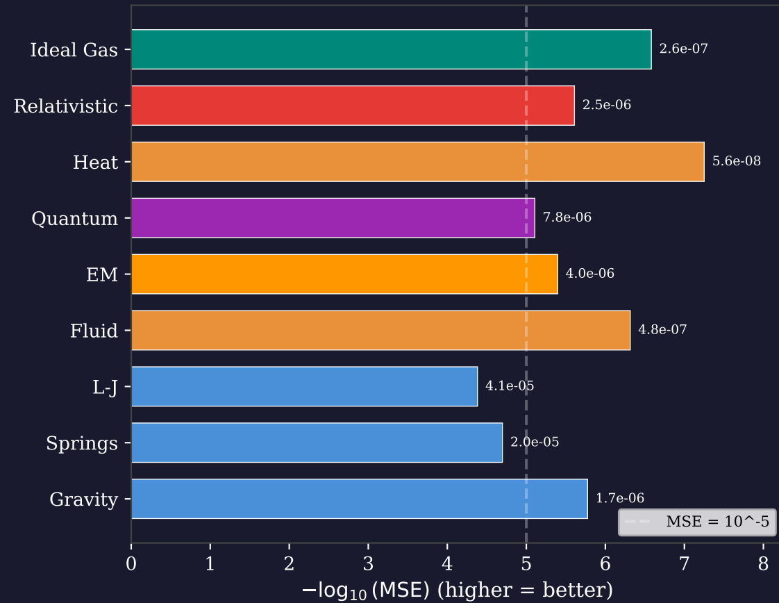
Test Performance Across 9 Physics Domains
