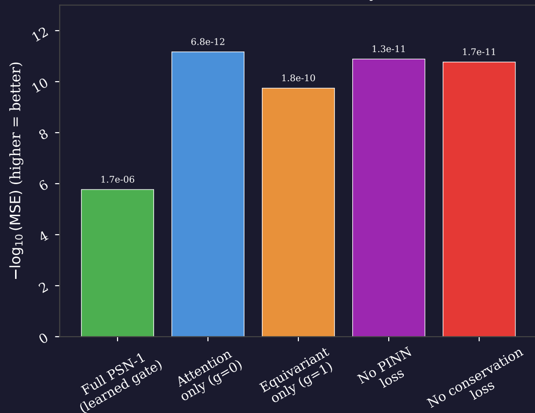
Prediction Accuracy
