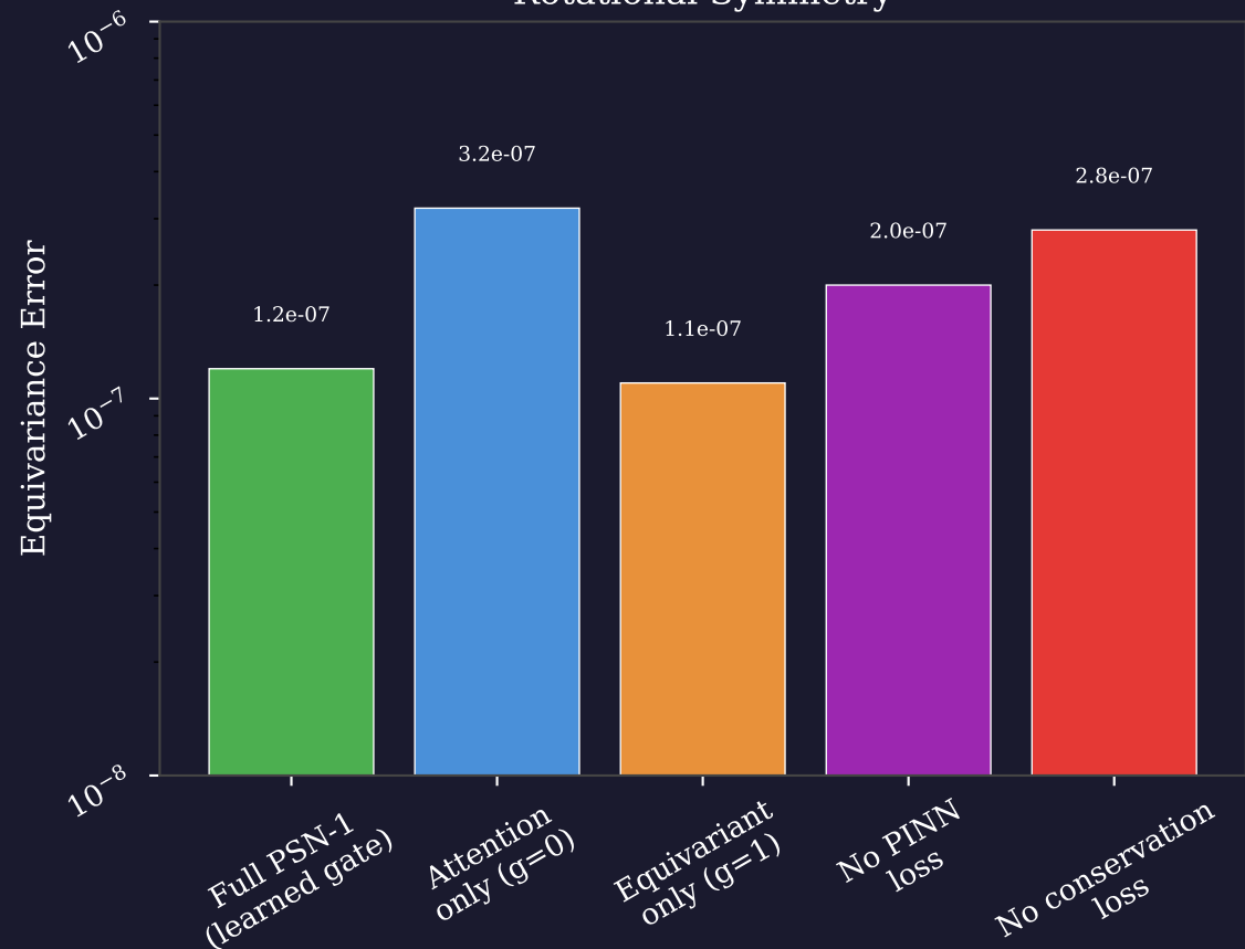
Rotational Symmetry
