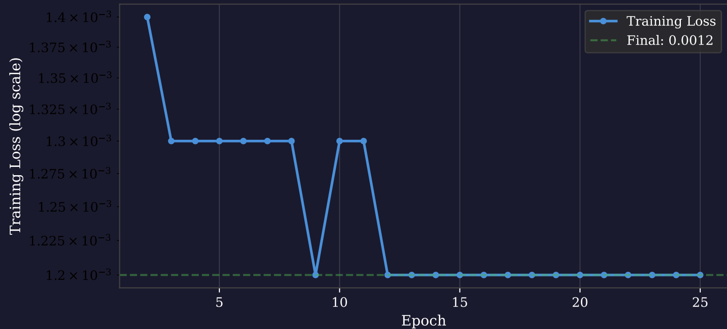
Training Convergence (25 epochs, 326s on T4 GPU)
