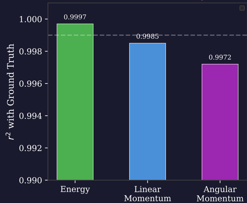
Conservation Discovery
