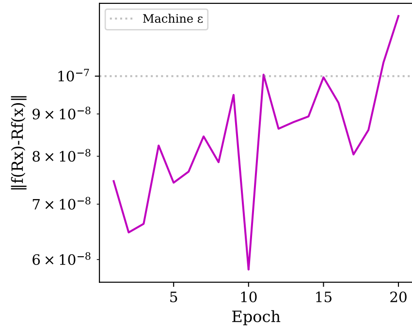
(c) Equivariance Error
