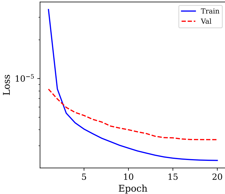
(a) Gravity Training
