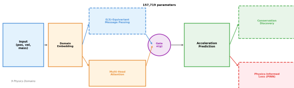
Figure 1: PSN-1 Architecture. Input particles feed into a domain embedding layer, then split into two pathways: E(3)-equivariant message passing (blue, dashed) and multi-head graph attention (orange). A learned gate \sigma(g) blends the two. The physics-informed loss and conservation discovery modules operate on the predicted acceleration. Total parameters: 157,719.
