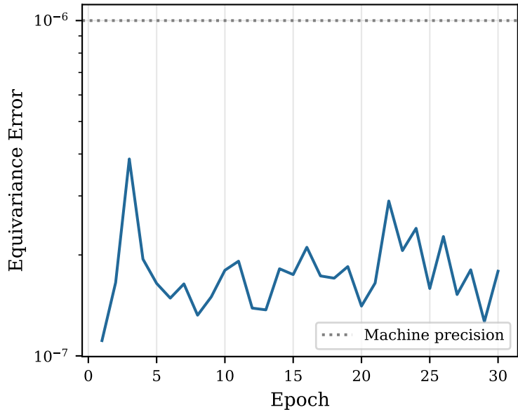
Equivariance Over Training (Gravity)
