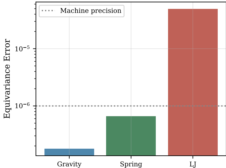
E(3) Equivariance Verification
