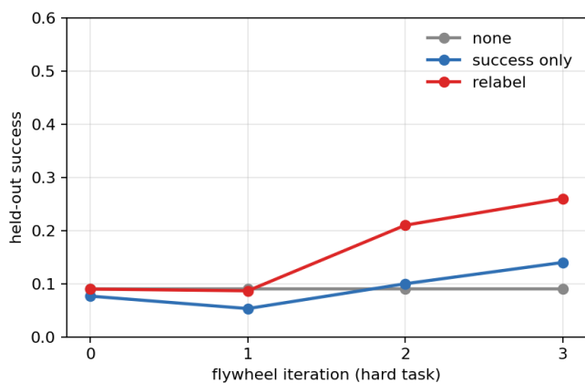
Fig. 6. Difficulty robustness: held-out success on the harder task. Relabeling still compounds; no feedback stays flat.
