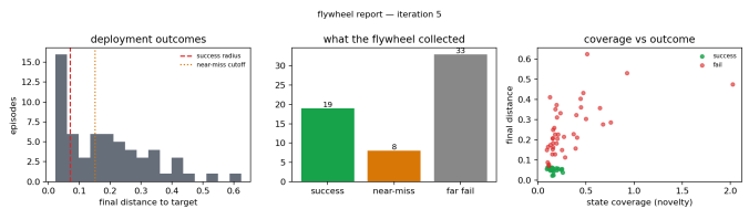
Fig. 2. The flywheel report for relabel_curated ’s final iteration: deployment outcomes, outcome buckets, and the coverage-vs-outcome that drives novelty-aware curation. Every number is committed under results/ .
