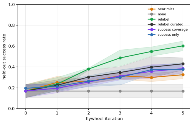
Fig. 1. Held-out push success vs. flywheel iteration (mean \pm std over 4 seeds). Oracle relabeling compounds; self-curation plateaus; the frozen control is flat.
