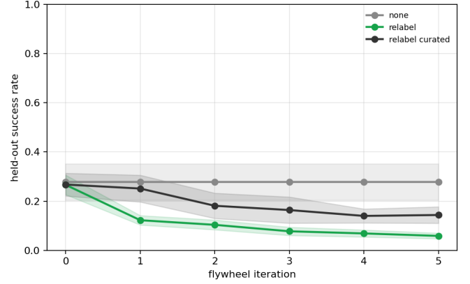
Fig. 8. Perception-grounded flywheel: held-out success vs. iteration for the CNN policy on 64 \times 64 RGB observations. Blind relabeling crashes the high-capacity CNN ( 0.27 \rightarrow 0.06 ); curated relabeling degrades far less ( 0.27 \rightarrow 0.14 ).
