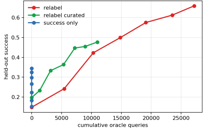
Fig. 5. Label efficiency: held-out success vs. cumulative oracle queries (main study). Curated relabeling spends less than half the queries of blind relabeling; self-curation spends none.
