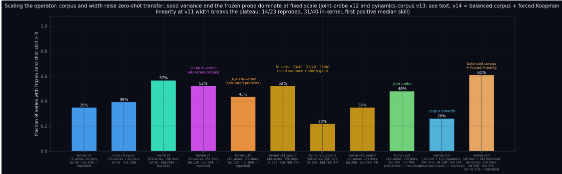
Figure 2: Scaling the operator: fraction of series with frozen skill > 0 on one shared 23-series corpus, same probe, eleven training budgets (v5 4k iters \rightarrow local 1.4k \rightarrow v7 15k \rightarrow v9 25k \rightarrow v10 60k, three v11 GPU seeds at latent 256/hidden 768, 25k, v12: the same capacity with the Koopman probe added to the pretraining loss, 25k, v13: latent 128/hidden 384 pretrained on 40 real series tiled with a 176-series dynamics battery, and v14: latent 256/hidden 768 on the re-balanced battery with the Koopman pretext at weight 2.5). Width and corpus raise transfer until the frozen-probe plateau; seed variance dominates thereafter, and neither joint-probe regularization (v12) nor dynamics-corpus breadth (v13) alone moves the curve — v13 instead trades smooth-periodic transfer for robustness on explosive series — while their combination (v14, balanced battery + forced Koopman linearity) breaks it: 14/23, the first run above the plateau.
