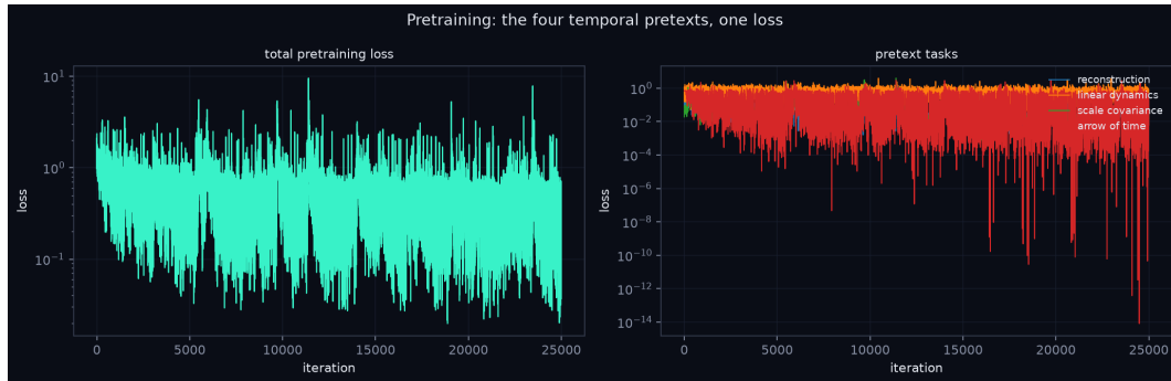
Figure 7: Pretext losses during the v7 Kaggle kernel pretraining.
