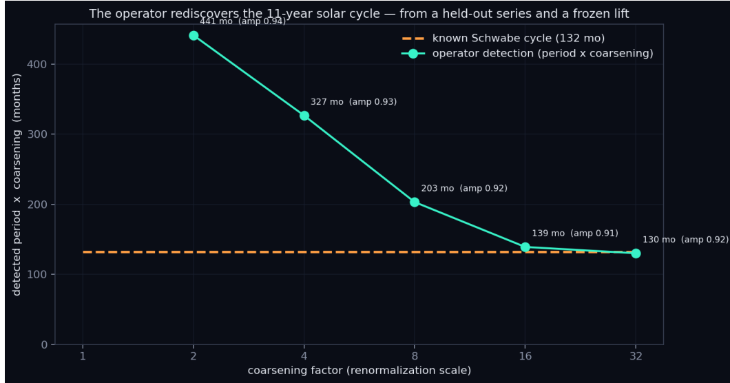
Figure 6: Scale-covariant period discovery on the held-out sunspot series: the frozen operator's detected period \times coarsening factor converges to the known 132-month Schwabe cycle.
