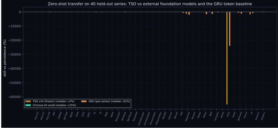
Figure 3: Zero-shot transfer on the 40-series protocol: TSO (v14, frozen) vs Chronos-t5-small (frozen) vs per-series GRU. Bars are skill vs persistence per series; medians in the legend. Chronos’s ~80k-series pretraining corpus transfers better on median; both foundation models beat the token baseline decisively.
