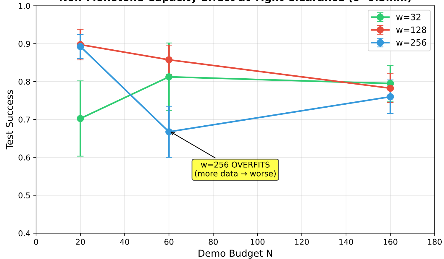
Non-Monotone Capacity Effect at Tight Clearance ( c=0.5\text{mm} )
