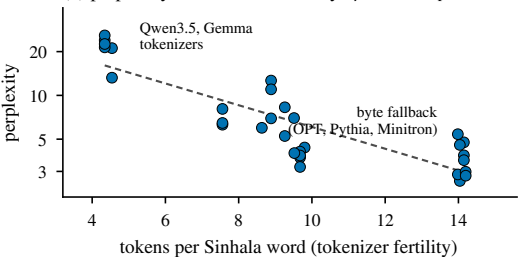
(b) perplexity vs. tokenizer fertility: \rho = -0.87 , p < 10^{-9}
