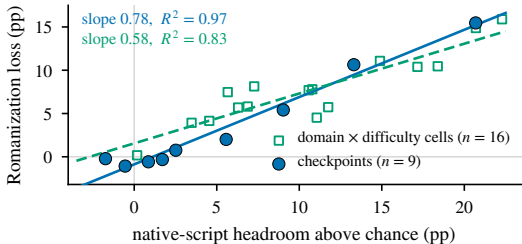
(a) the loss tracks native-script headroom
