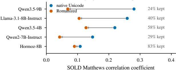
(b) offensive-language detection collapses
