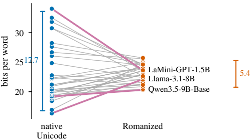
(a) 31 checkpoints, language modelling cost
