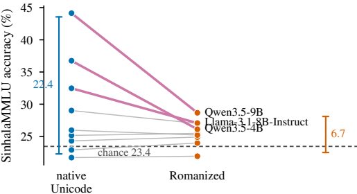
(b) 9 instruction-tuned checkpoints, accuracy
