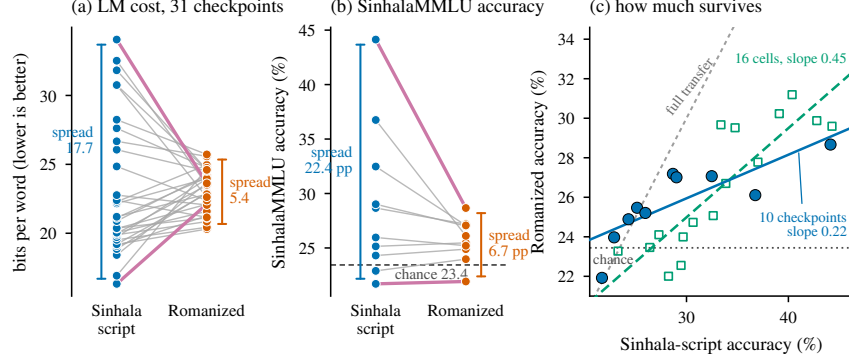
Figure 1: (a) Bits per word, comparable across columns since word counts match within a pair. Highlighted lines are cheaper on Romanized text. (b) SinhalaMMLU accuracy. (c) The same numbers as levels, with the 16 domain by difficulty cells. Both slopes fall well below the full-transfer slope of 1. LaMini-GPT-1.5B, unparseable on 95.9% of Sinhala-script items, is omitted from (b) and (c).
