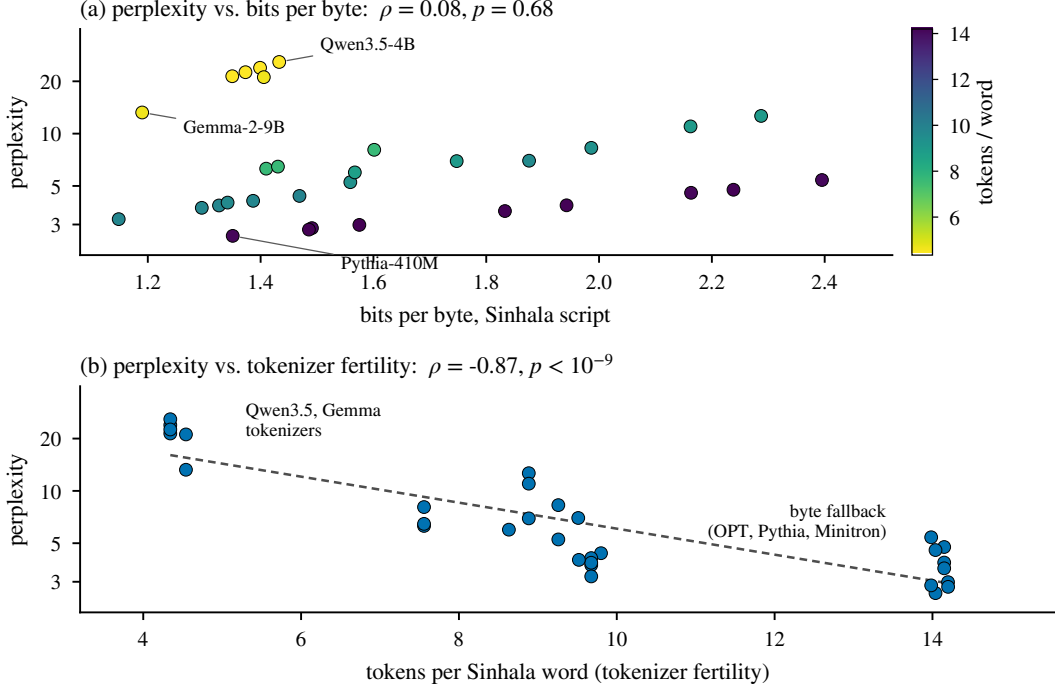
Figure 2: (a) Sinhala-script perplexity against Sinhala-script bits per byte over 31 checkpoints. The two are unrelated ( \rho = 0.08, p = 0.68 ). (b) Perplexity against tokenizer fertility, which explains it almost fully ( \rho = -0.87, p < 10^{-9} ).
