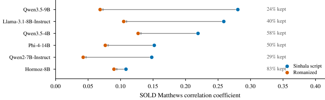
Figure 5: SOLD under romanization. Accuracy moves a few points against a 59.4% majority baseline while Matthews correlation loses a median 55% of its value.
