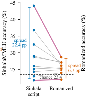
(b) SinhalaMMLU accuracy
