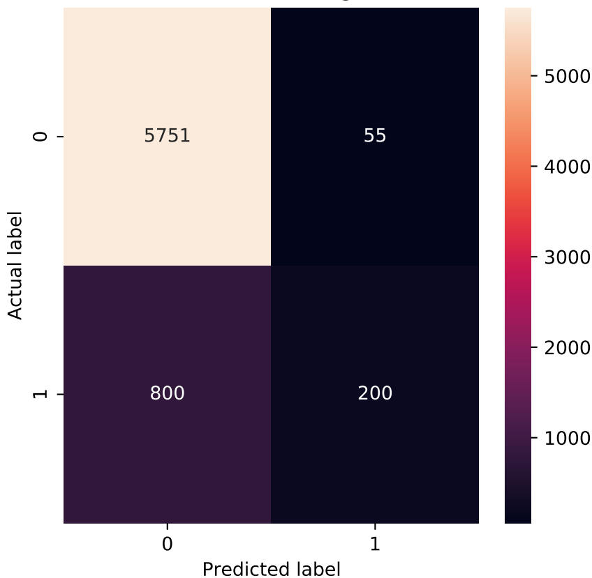
Confusion matrix @0.50
