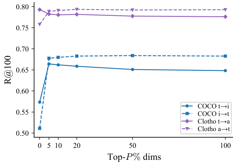
(b) Selective PMC (top-P %)
