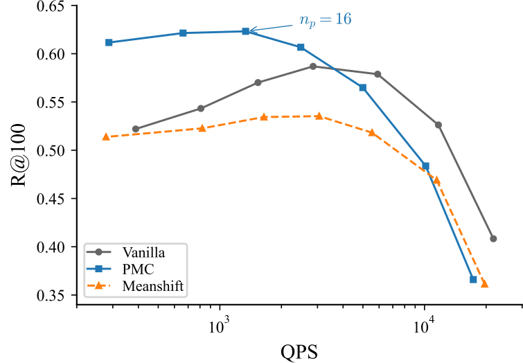
(c) R@100–QPS Pareto
