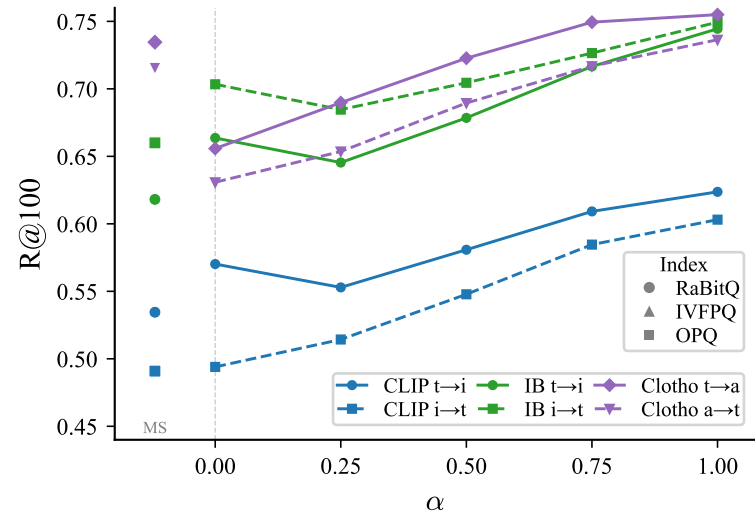
(a) Sign-bit: \alpha sweep
