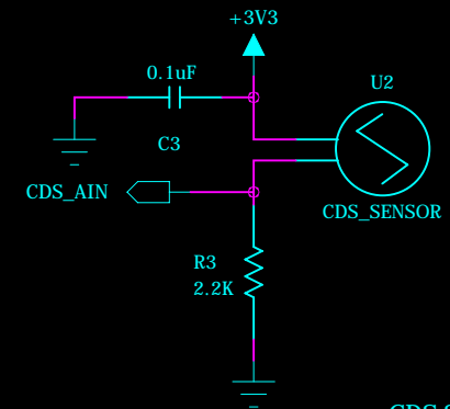
CDS Sensor
