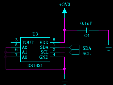
Digital Temperature Sensor
