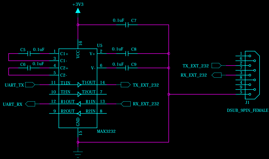
UART Driver & Connector
