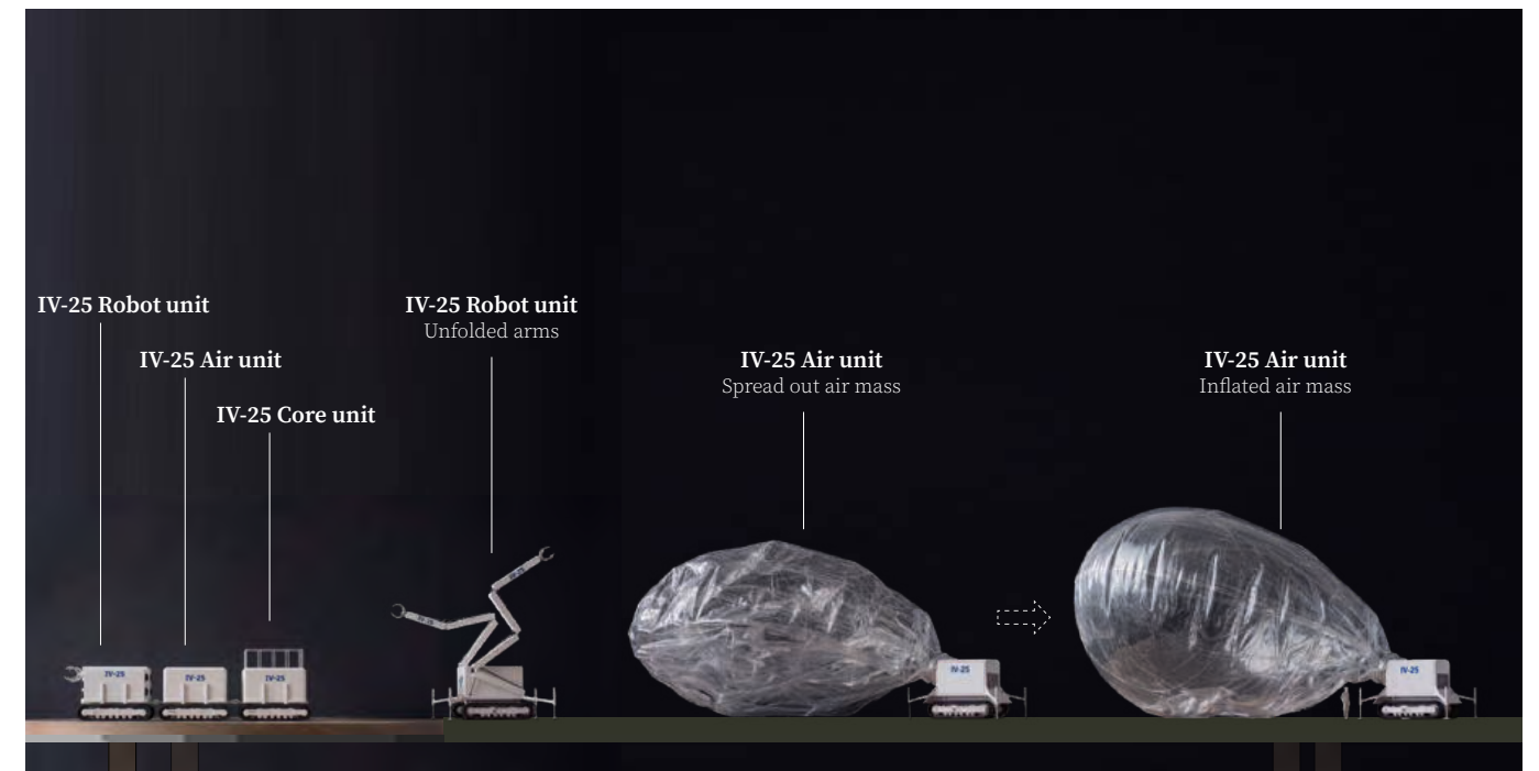
Photo. 1:50 model
