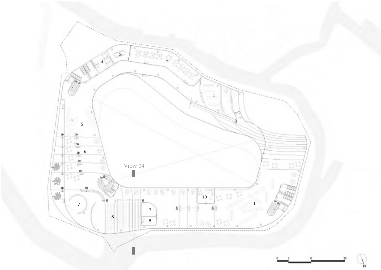
2nd Floor Plan 1 : Library 2 : Teacher's room 3 : Meeting room 4 : Nursing room 5 : Lounge 6 : Complex Hall 7 : Music classroom 8 : Auditorium 9 : Studio 10 : Counseling room
