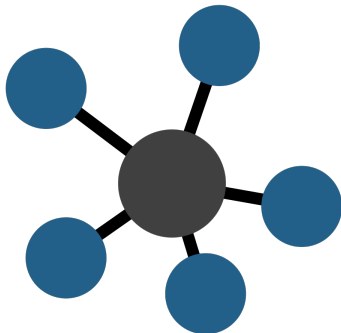
Graph theory
