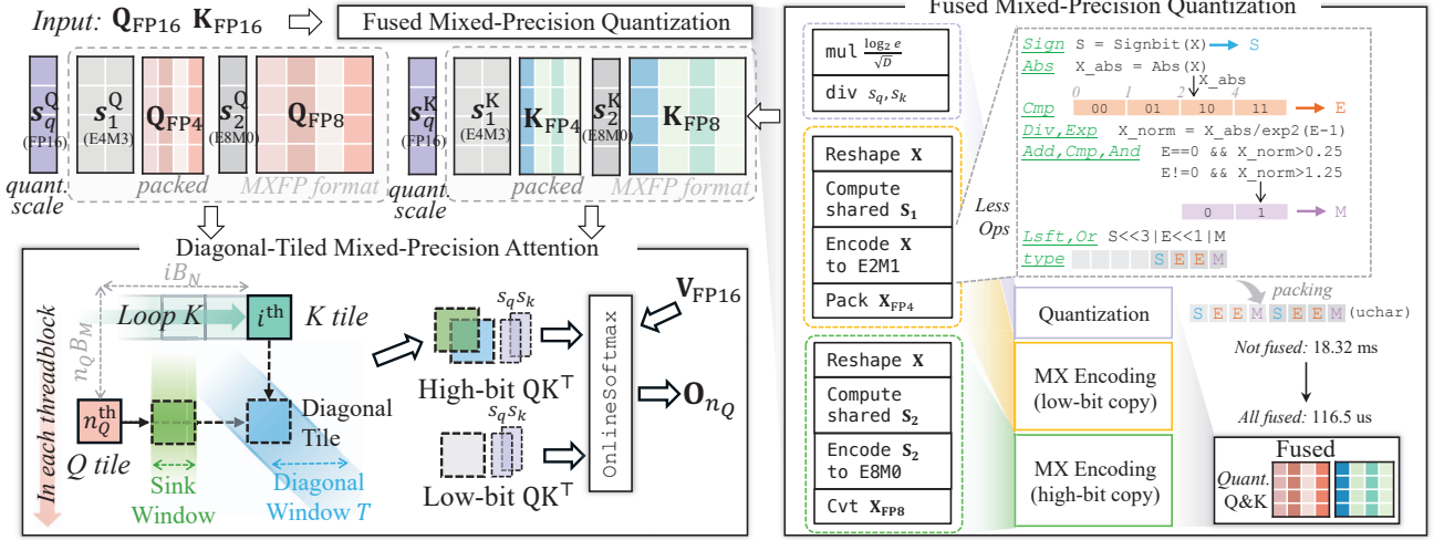
Figure 2. Overview workflow of our Diagonal-Tiled Mixed-Precision Attention. It first applies fused mixed-precision quantization to produce low-bit and high-bit Q and K representations, and then performs diagonal-tiled mixed-precision attention, using higher precision near the diagonal and lower precision elsewhere to balance accuracy and efficiency.
