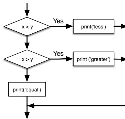
Figure 3.3: If-Then-ElseIf Logic
