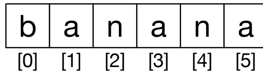
Figure 6.1: String Indexes
