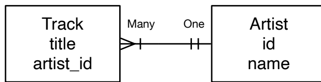
Figure 15.4: A Verbose One-to-Many Data Model
