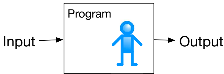
Figure 14.1: A Program
