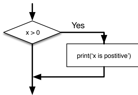
Figure 3.1: If Logic
