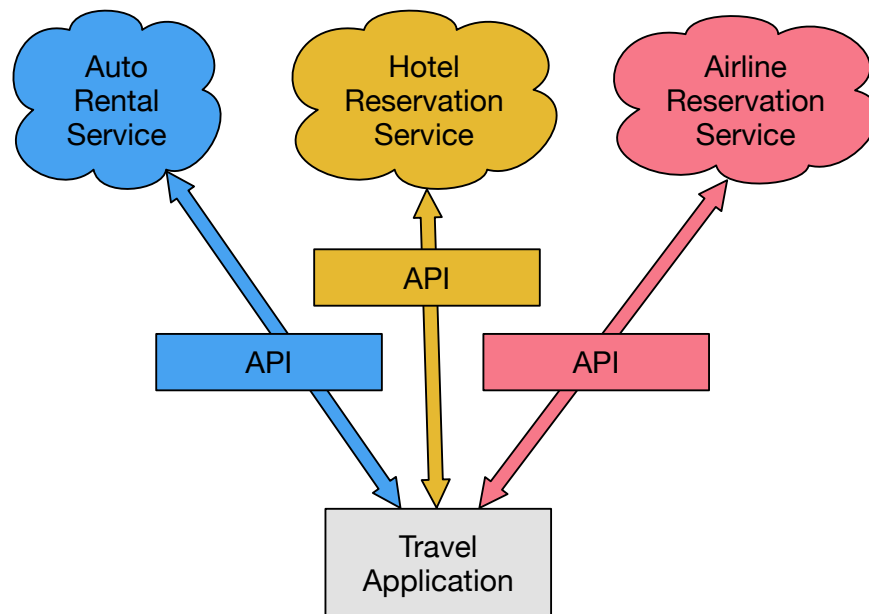
Figure 13.2: Service-oriented architecture
