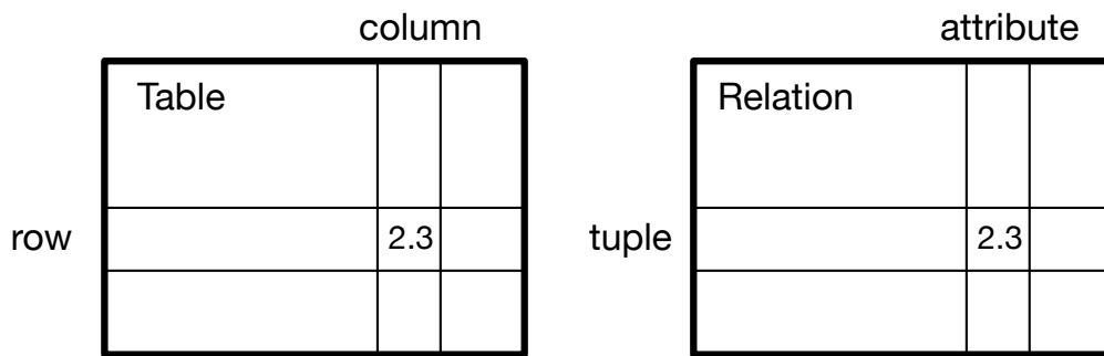
Figure 15.1: Relational Databases
