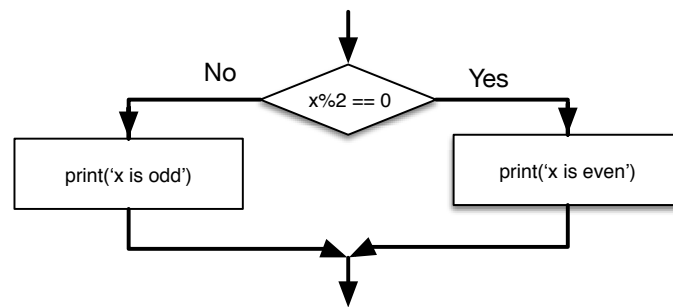
Figure 3.2: If-Then-Else Logic
