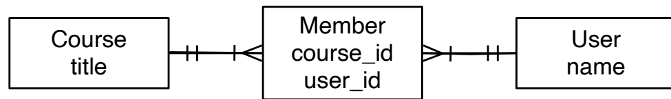
Figure 15.8: A Many to Many Connector Table
