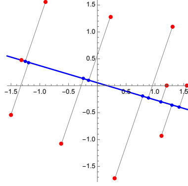
Figure 4: A 2D synthetic data cloud with PC_1 . This is the same dataset visualized as points on the boundary of the PSD cone in Figure 3. The blue line is \text{Span}(\mathbf{v}) where the blue dot in Figure 3 is the point \mathbf{v}\mathbf{v}^\top .
