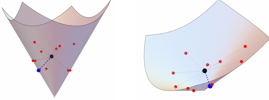
Figure 3: The same PSD cone as above (two views), with the same red points and their average in black. The projection of S to the boundary is marked in blue. This is the best rank one approximation, which finds the top principal component of the data behind the red points.
