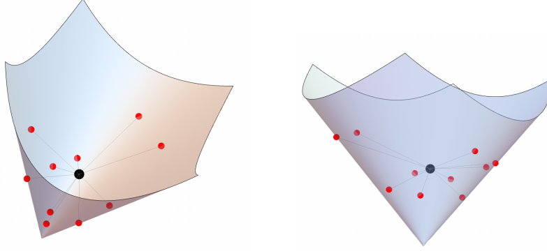
Figure 2: The 2 \times 2 PSD cone (two views), i.e. (a, b, c) \in \mathbb{R}^3 with a, c \geq 0 , ac \geq b^2 . Its boundary consists of matrices \mathbf{v}\mathbf{v}^\top for \mathbf{v} \in \mathbb{R}^2 . Here 10 mean-centered points (say \mathbf{v}\mathbf{v}^\top for \mathbf{v} \in \{\mathbf{x}^{(1)}, \dots, \mathbf{x}^{(n)}\} ) on the boundary are shown in red. Their average (in black) is the sample covariance matrix of the data \mathbf{x}^{(1)}, \dots, \mathbf{x}^{(n)} .
