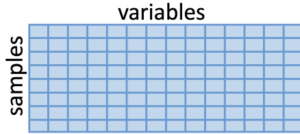
Figure 1: A data matrix, samples as rows, variables as columns
