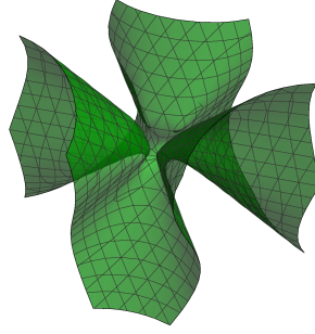
Figure 3: An example of a cubic surface
