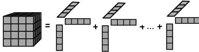
Figure 1: A tensor written as a sum of outer products of vectors.
